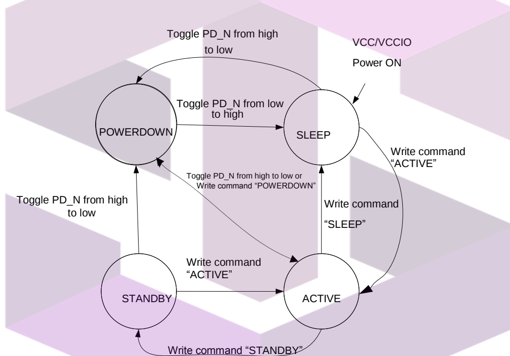
Figure 4-11 Power State Transition
